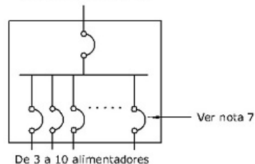
DIAGRAMA UNIFILAR
