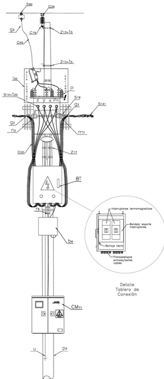
VISTA FRONTAL
