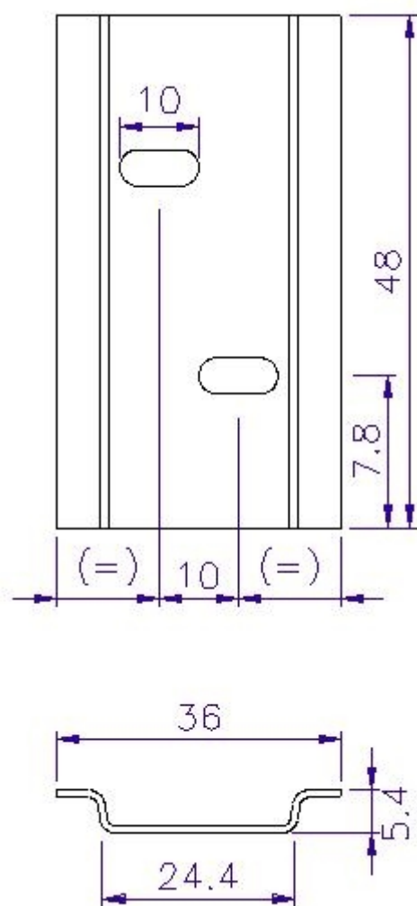
FIGURA 10. RIEL INTERRUPTOR
